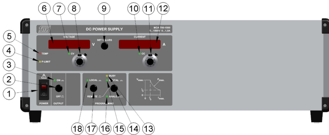
Front panel shown for illustrative purposes only, dimensions and layout differ by power rating - see mechanical details table.
