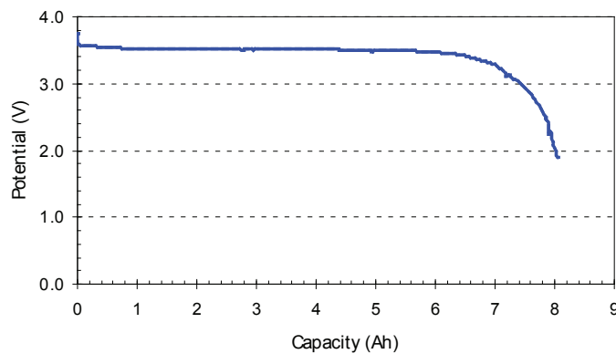
Discharge at 30 mA, 120°C
